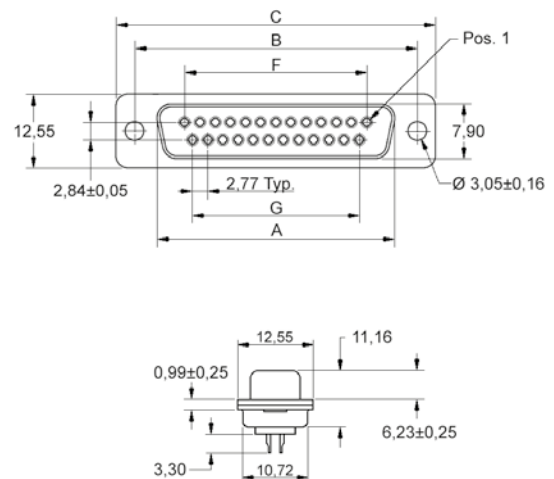
Socket connector
