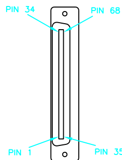
FRONT VIEW OF 68 W CONNECTOR
