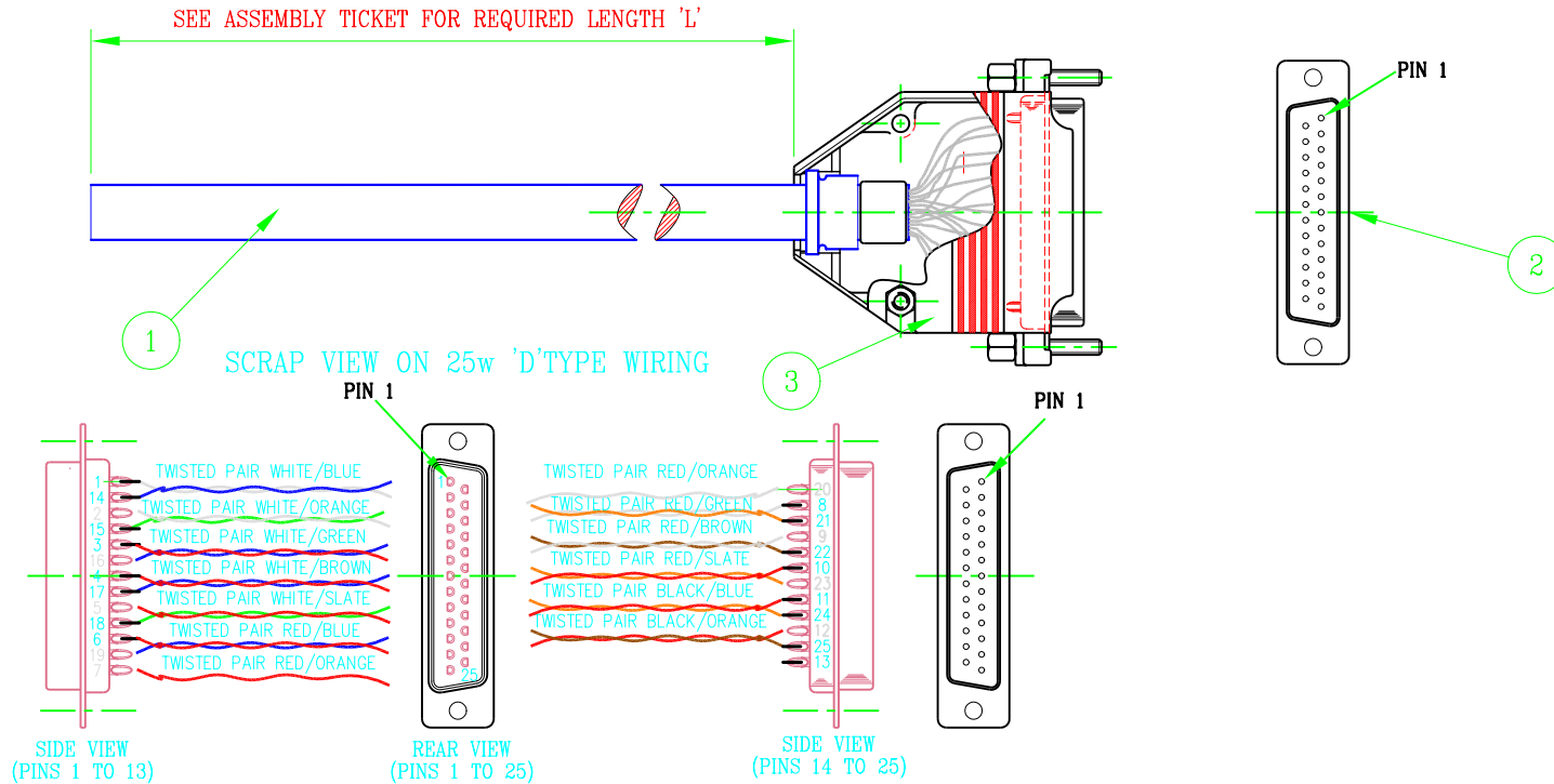
DETAIL 1 CABLE PREPERATION
