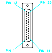
REAR VIEW OF 25 W "D" CONNECTOR
