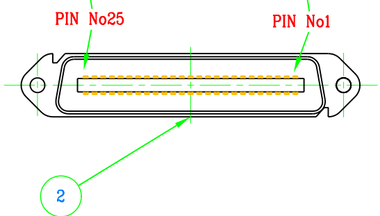
CONNECTOR AMPCHAMP 50w MALE
