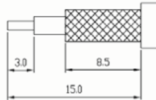
Recommended Stripping Dimensions
