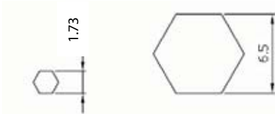
Die Size A Die Size B Recommended Stripping Dimensions
