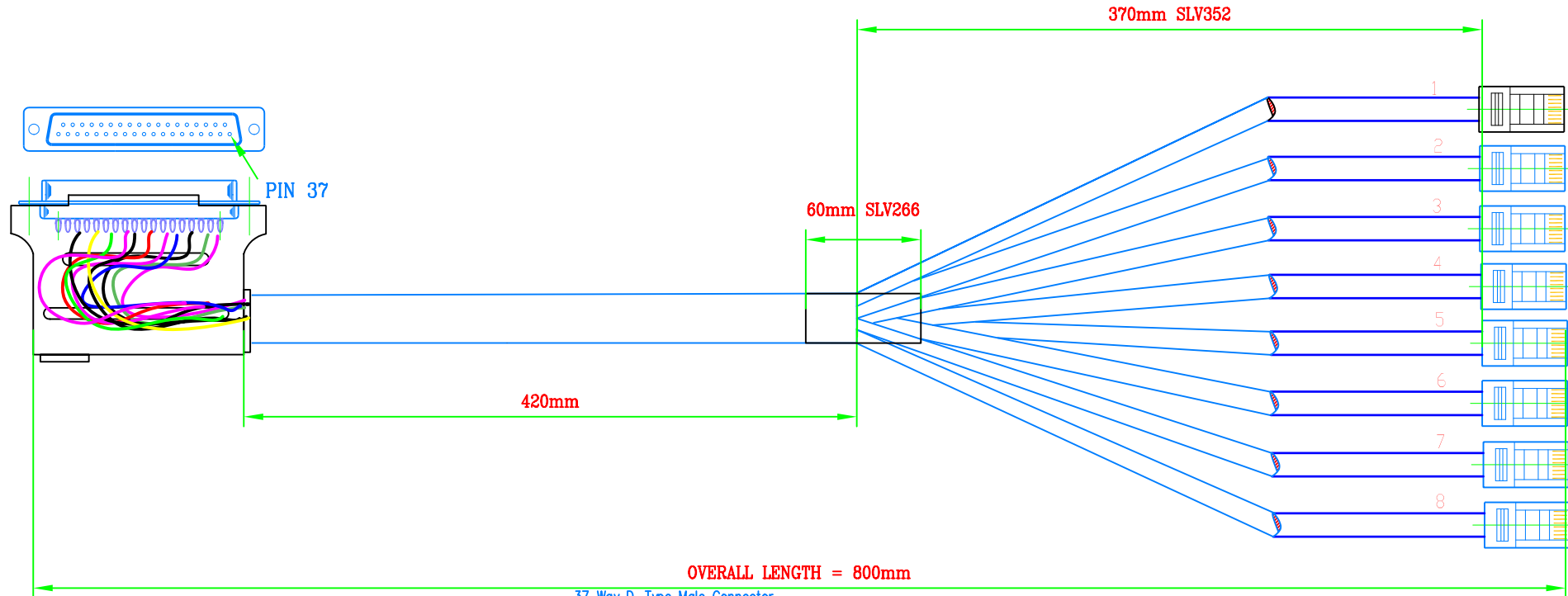
37 Way D-Type Male Connector
